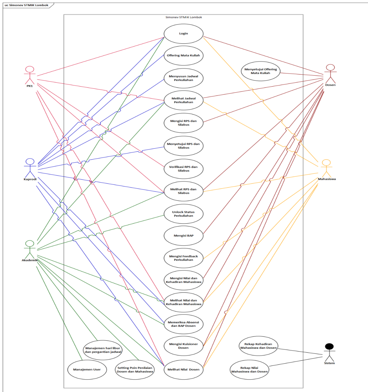
Gambar 6. Use Case Diagram
