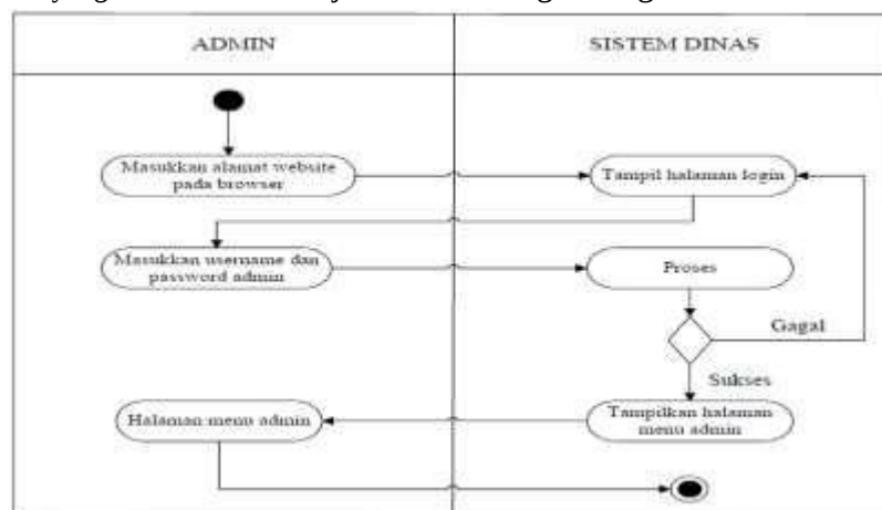
Gambar 4. Activity Diagram Login Admin
