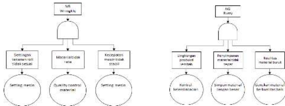
Gambar 4. Fault Tree Analysis NG Wrinkle dan NG Rusty
