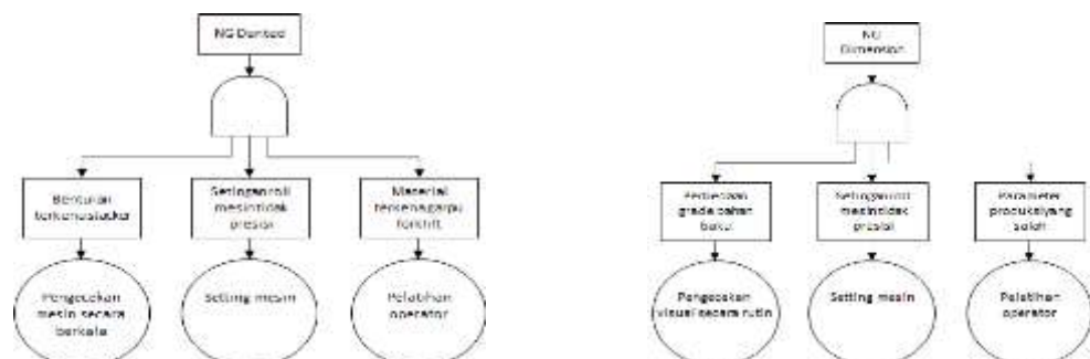
Gambar 3. Fault Tree Analysis Dented dan NG Dimension
