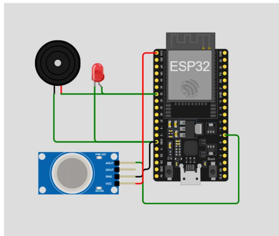
Gambar 3. Wiring Hardware
