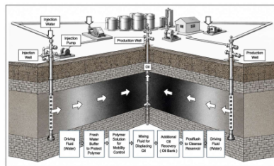
Gambar 1. Ilustrasi mekanisme polymer flooding.
