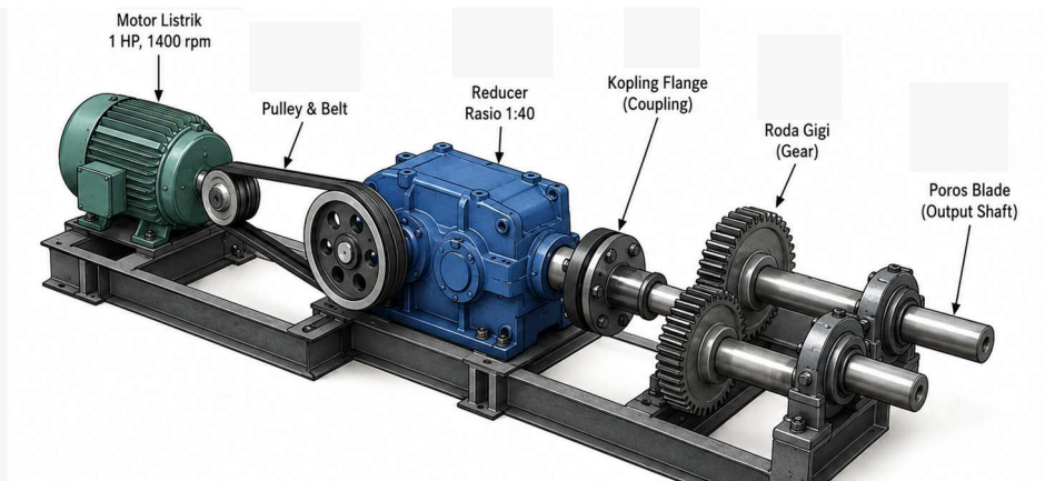
Gambar 3. Layout sistem transmisi motor, pulley-belt, reducer, kopling, roda gigi, dan poros blade.
