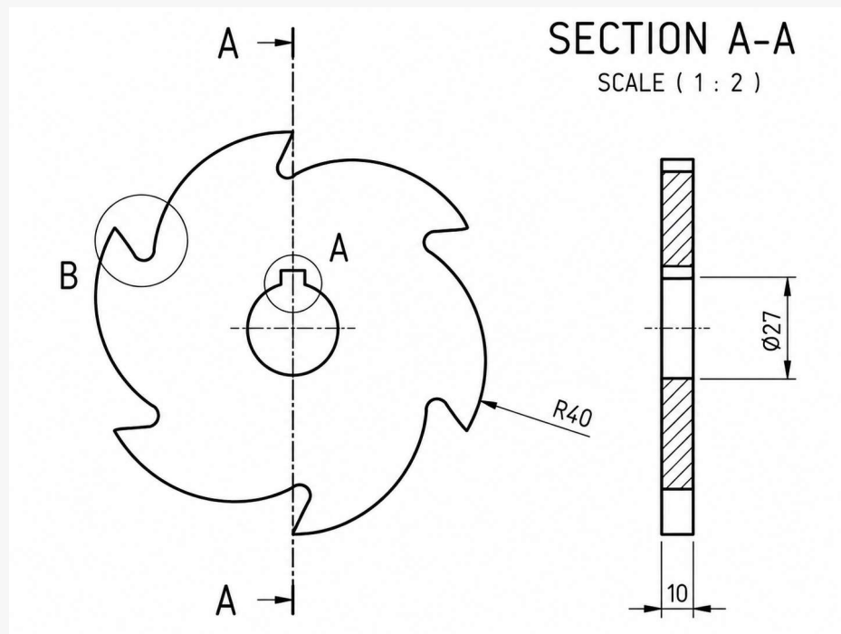
Gambar 4. Blade/mata pisau rotary cutter
