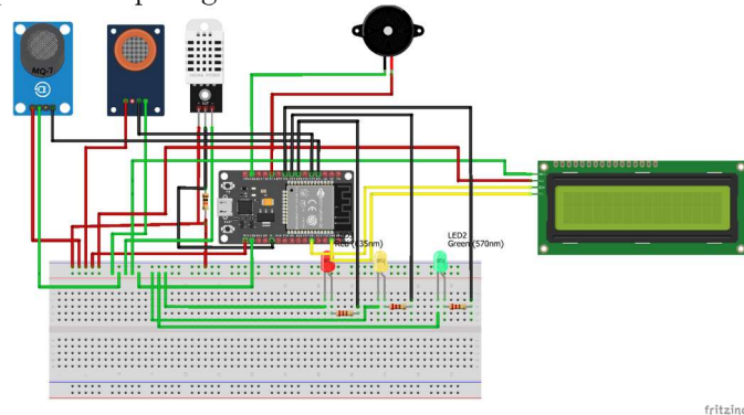
Gambar 3. Diagram Wiring Alat
