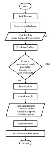
Gambar 3. 1 Diagram Alir
