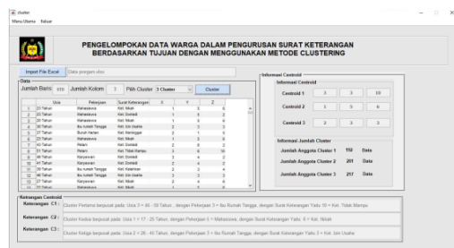
Gambar 2. Proses Cluster
