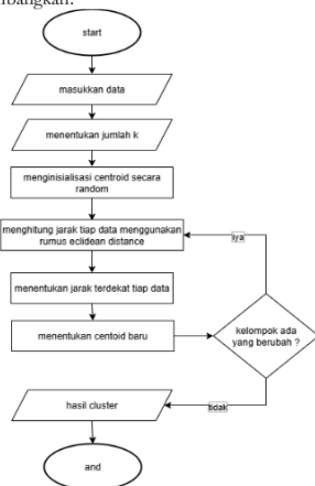
Gambar 1. Flowchart Algoritma K-Means
