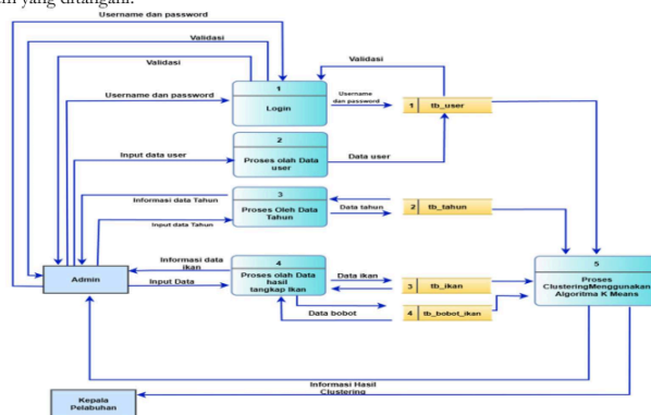
Gambar 2. Data Flow Diagram level 1
