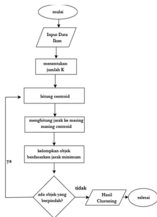
Gambar 1. Flowchart K Means.
