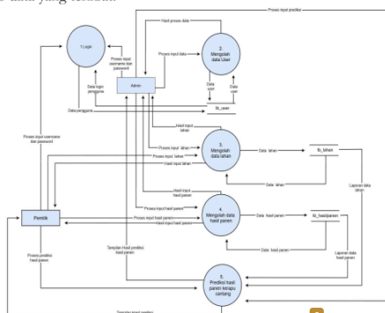
Gambar 2. Data Flow Diagram Level 1.
