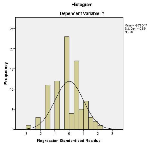
Gambar 7. Histogram Residual
