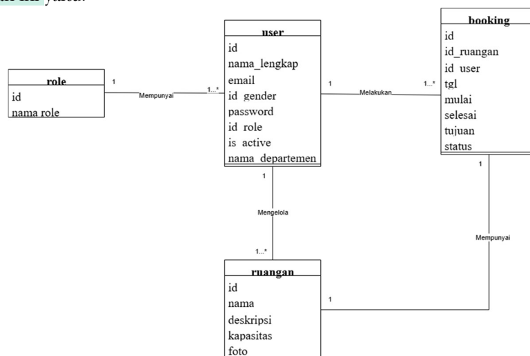
Gambar 4. Class Diagram
