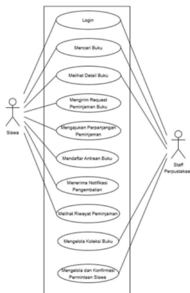
50 Gambar 2. Use Case Diagram.
