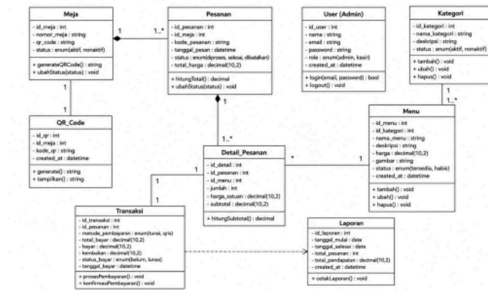
Gambar 3. 4 Class Diagram
