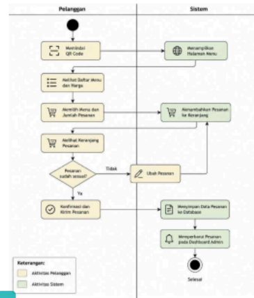
Gambar 3. 3 Activity Diagram
