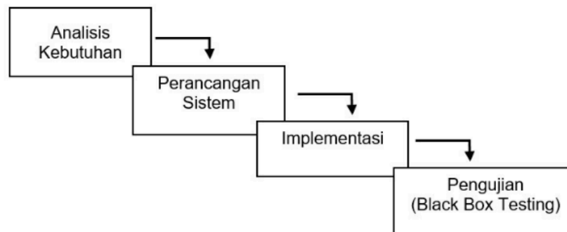
Gambar 3.1. Model Waterfall
