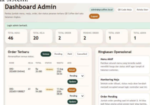
Gambar 4. 4 Dashboard Admin
