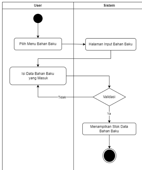
Gambar 4. Activity Diagram Bahan Baku Masuk.
